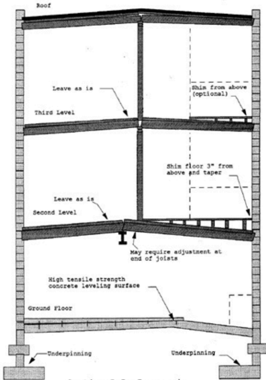
Section D-D: Proposed
